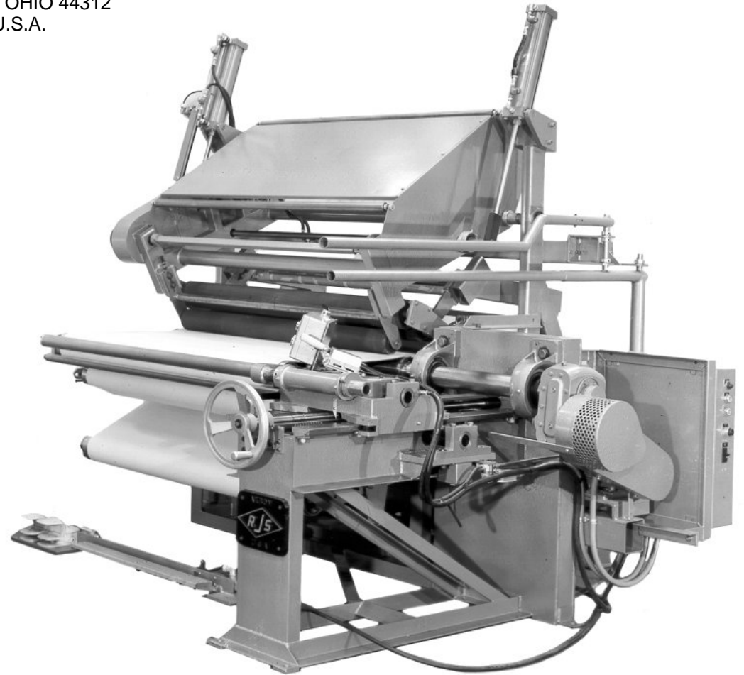
MODEL A BAND BUILDER WITH MODEL 107 GUM LET-OFF AND MODEL 103 FABRIC SERVICER (MOTOR SIDE)
